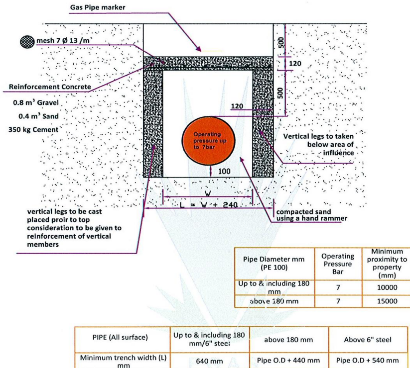
Figure 2-5: Typical layout of U-shaped concrete slab (Source: EGAS technical drawings)
