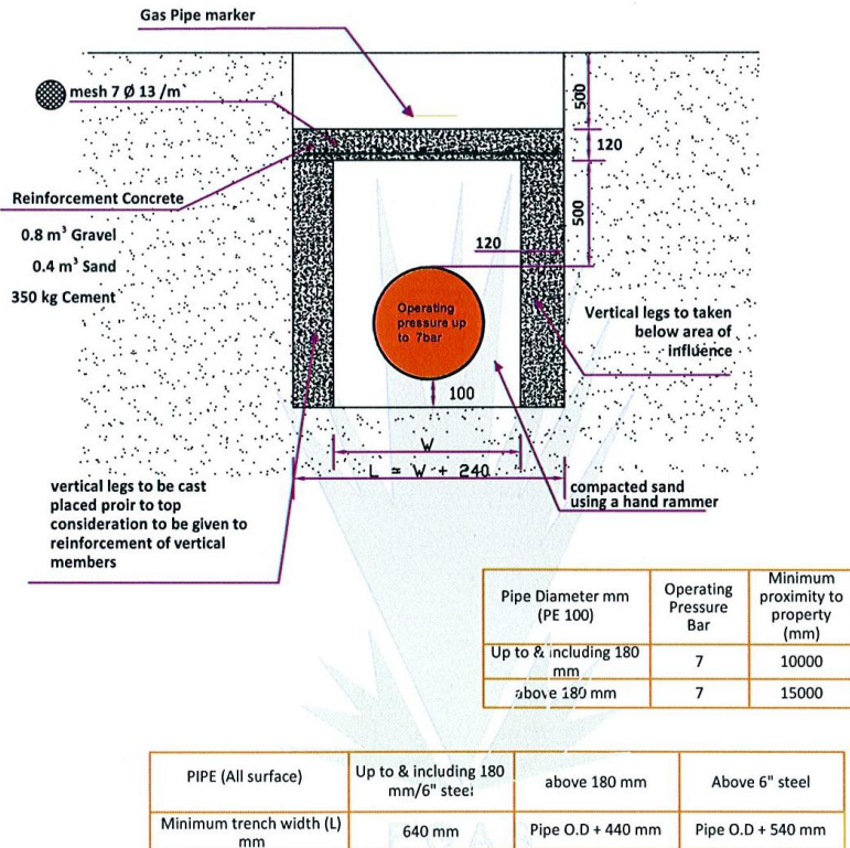
Figure 2-3: Typical layout of U-shaped concrete slab (Source: EGAS technical drawings)
