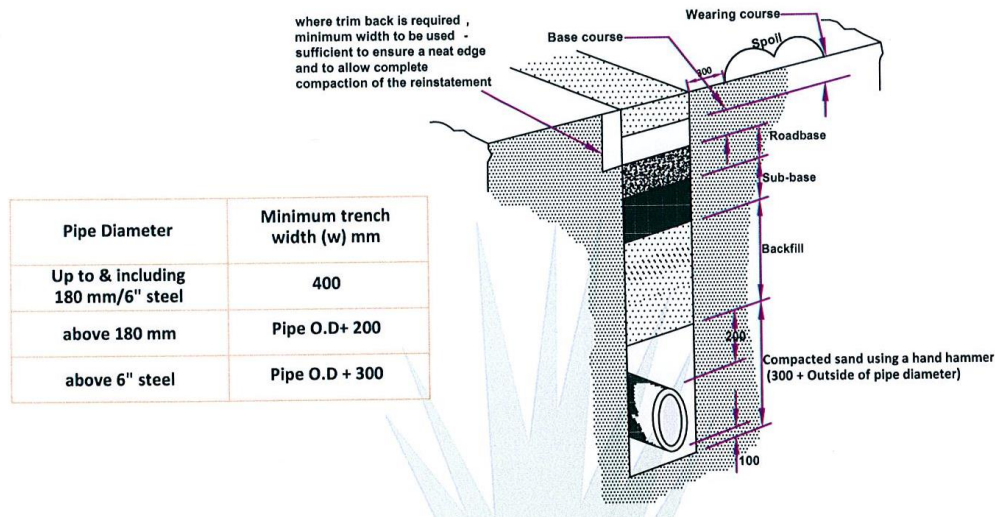
Figure 2-2: Typical backfill arrangement (Source: EGAS technical drawings)
