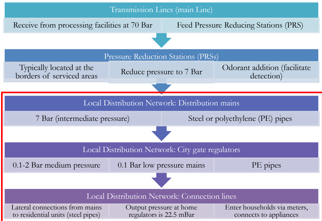
Figure 2-1: General components of the distribution network in the specific sites
