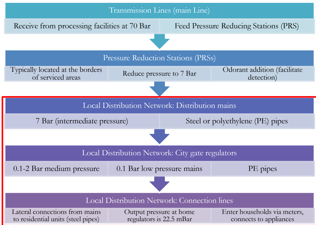
Figure 2-1: General components of the city’s distribution network
