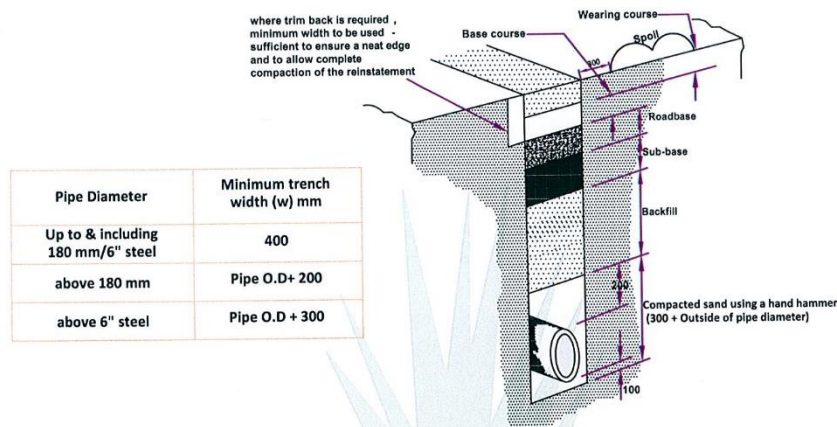
Figure 2-4: Typical backfill arrangement (Source: EGAS technical drawings)
