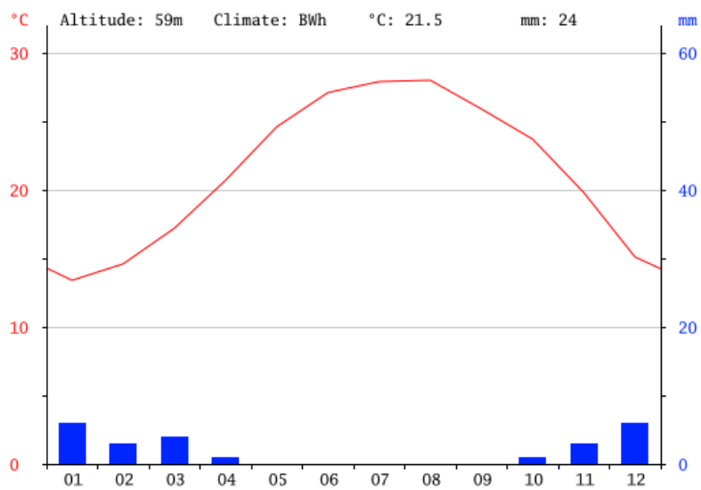
Figure 4-4: Average rainfall
