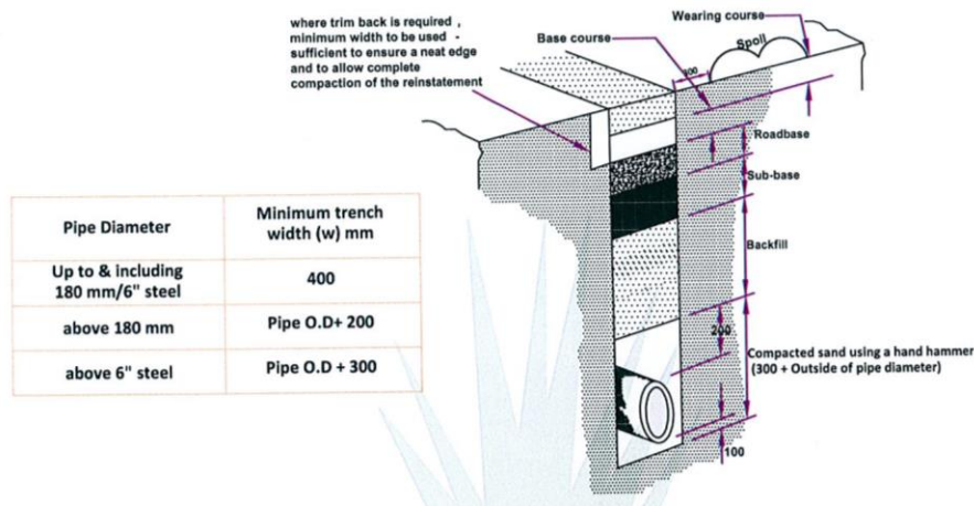
Figure 2-4: Typical backfill arrangement (Source: EGAS technical drawings)
