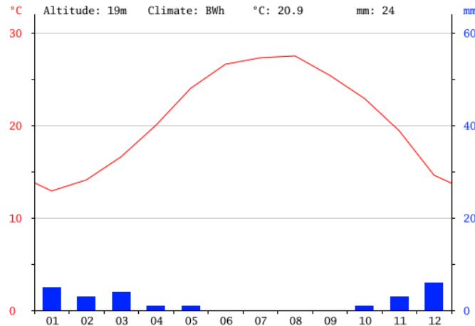
Figure 4-3: Average rainfall in Shebin Al Qanater 6
