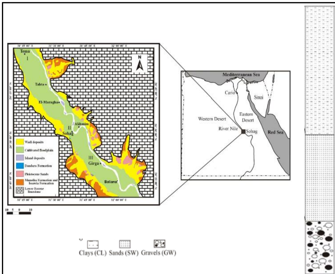
Figure 4-4: Soil composition. Sohag city lies in the green area. Reference: Al Haddad and Shater, 1988.
