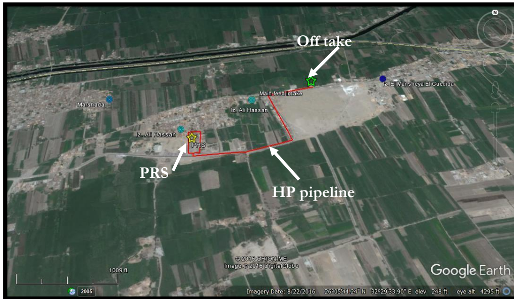
Figure 2-2: High pressure pipeline (red line) connecting main feed off-take (green star) to the PRS location (yellow star)
