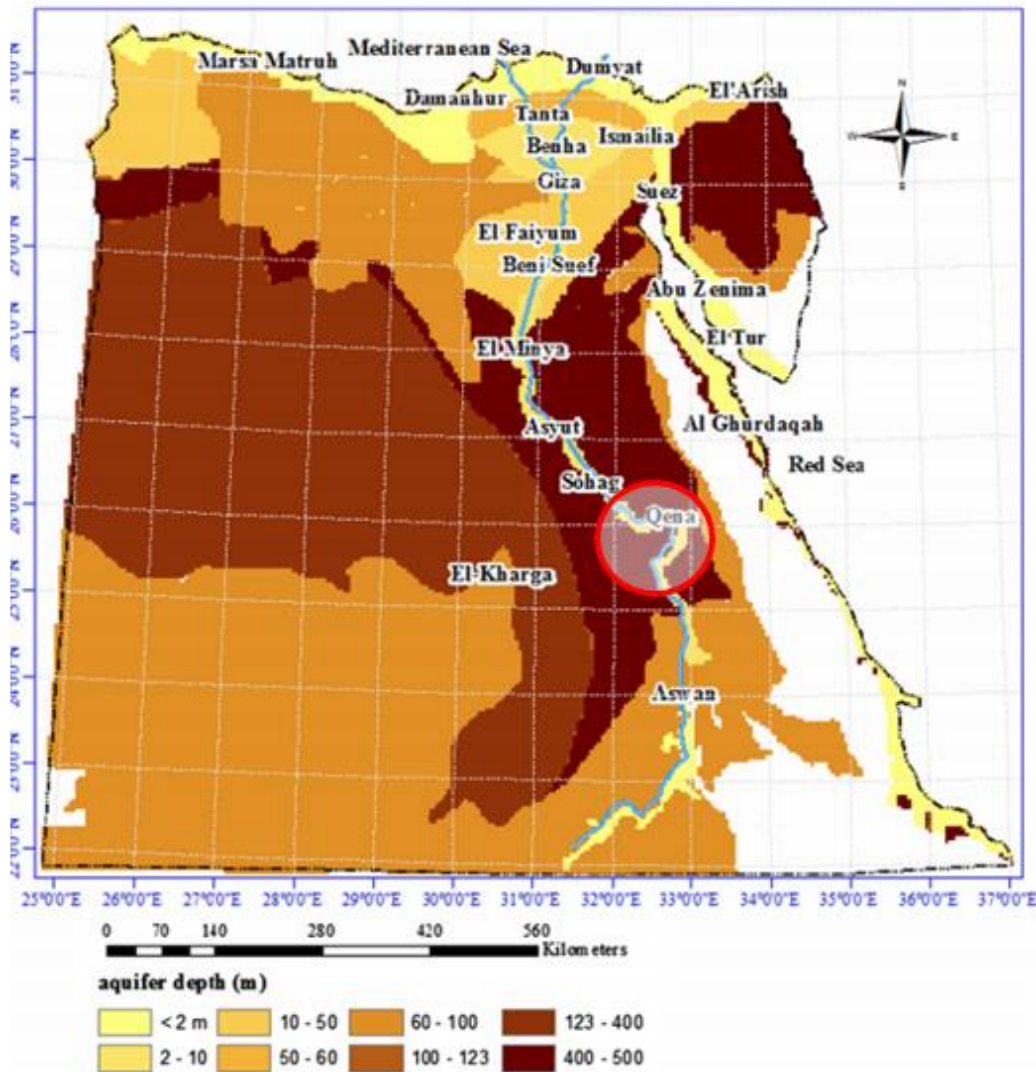
Figure 4-5: Aquifer depths
