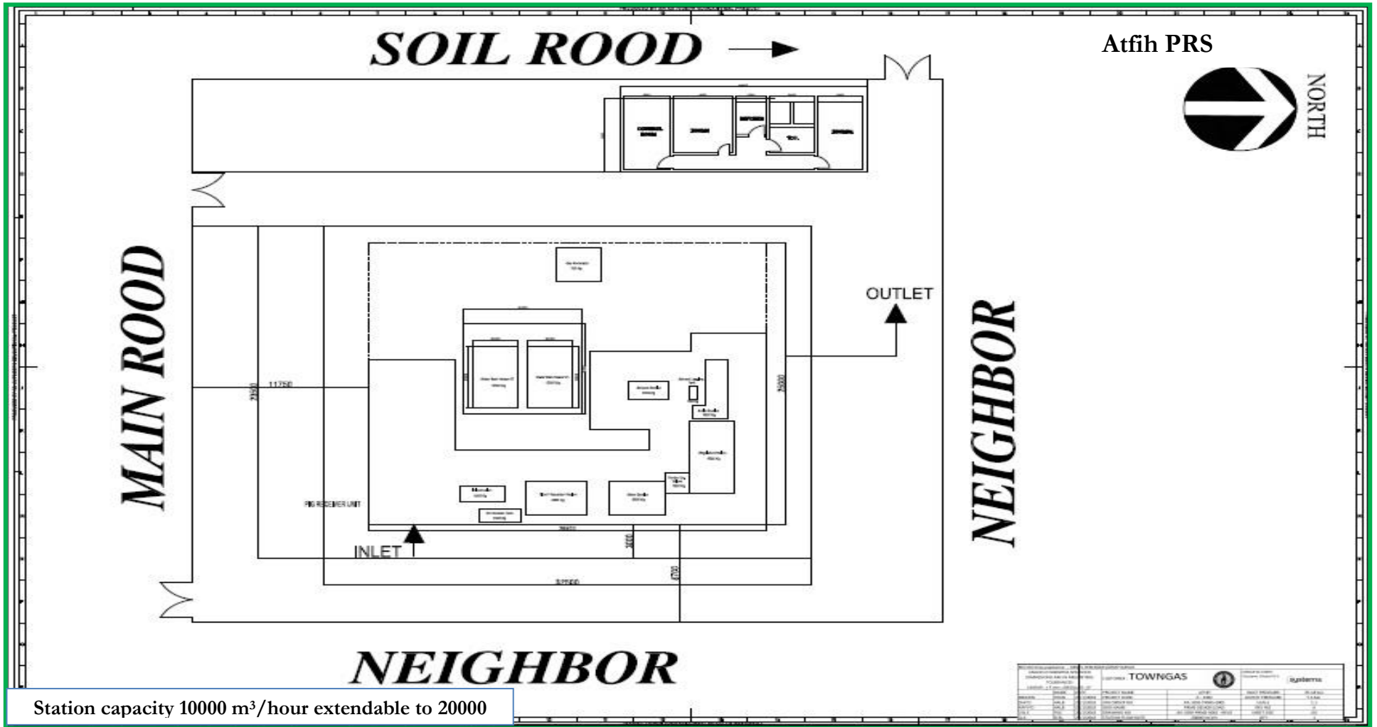
Figure 2-10: The proposed layout of Atfih PRS
