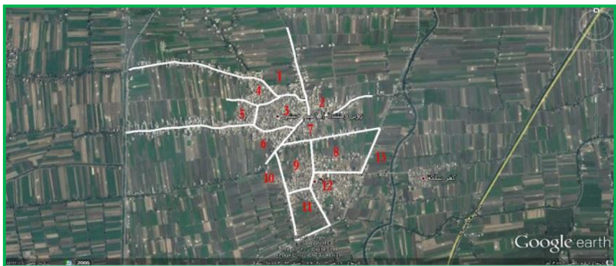
Figure 2-8: Satellite map showing the proposed distribution - network feeding Salaka area
