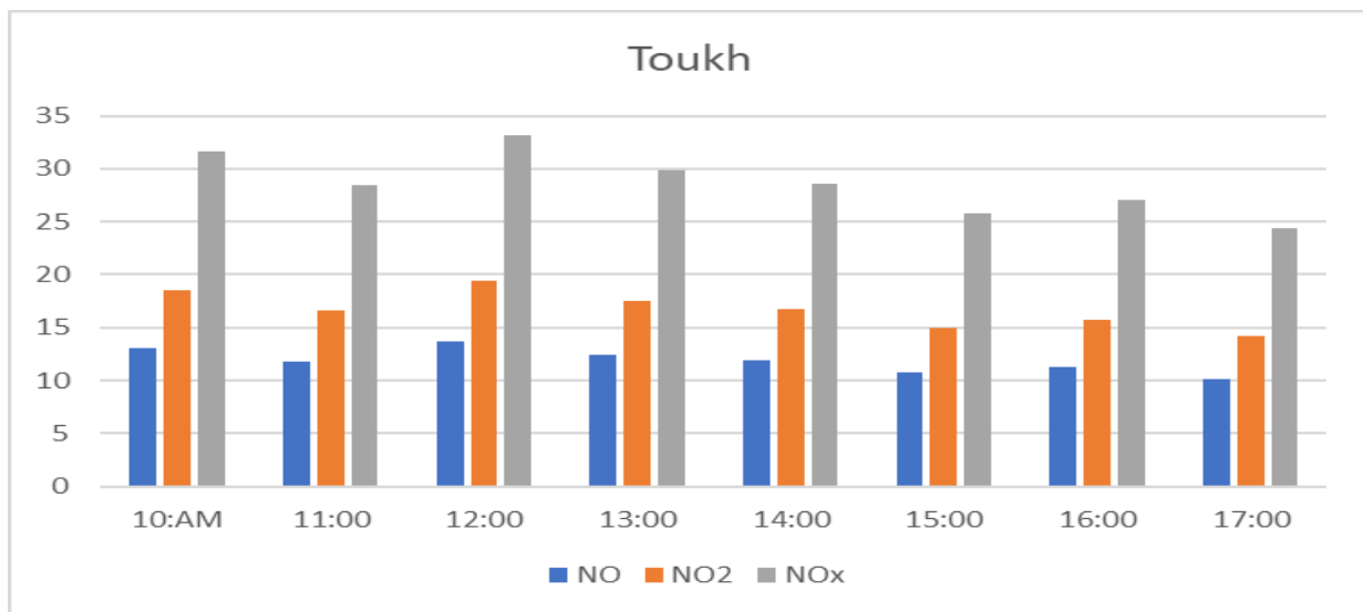
Figure 4-1 NO x variation in the location ( \mu\text{g}/\text{m}^3 )
