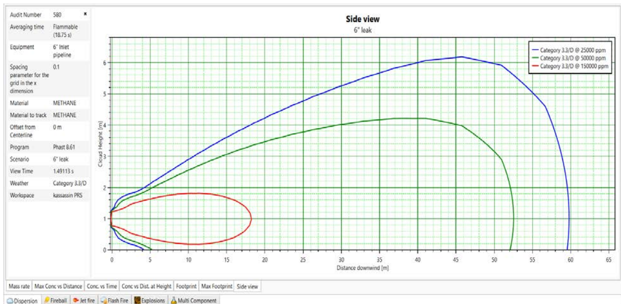
Figure 18. Gas Cloud Side View (UFL/LFL) (6'' Inlet Pipeline Full Rupture)
