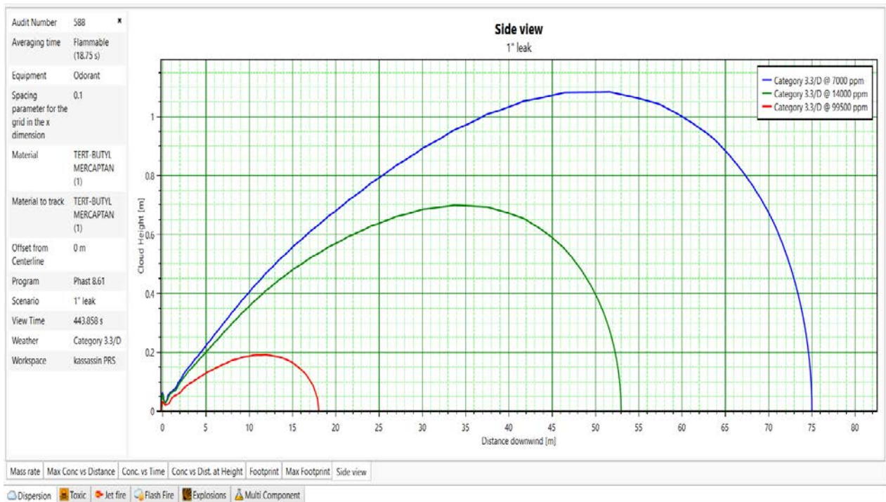
Figure 30. Vapor Cloud (UFL/LFL) Side View Graph (Odorant leak)
