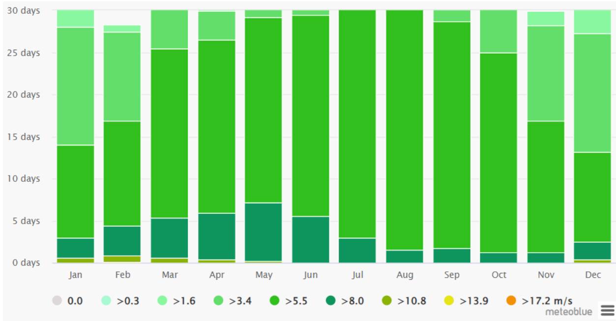
Figure 5. Monthly Variation of the Wind Speed for El- Kasasin Area
