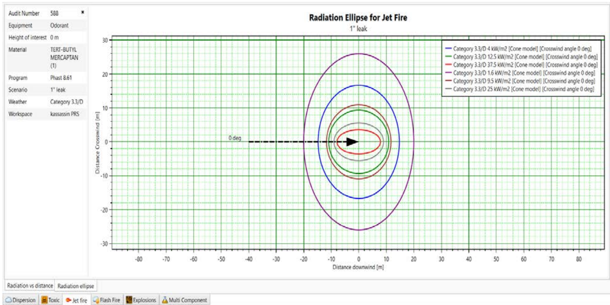
Figure 32. Heat Radiation Contours - Jet Fire Graph (Odorant Leak)
