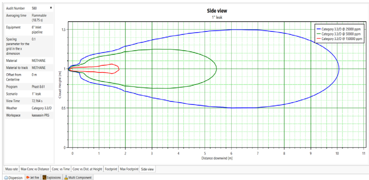
Figure 12. Gas Cloud Side View (UFL/LFL) (1" hole in 6" Inlet Pipeline)
