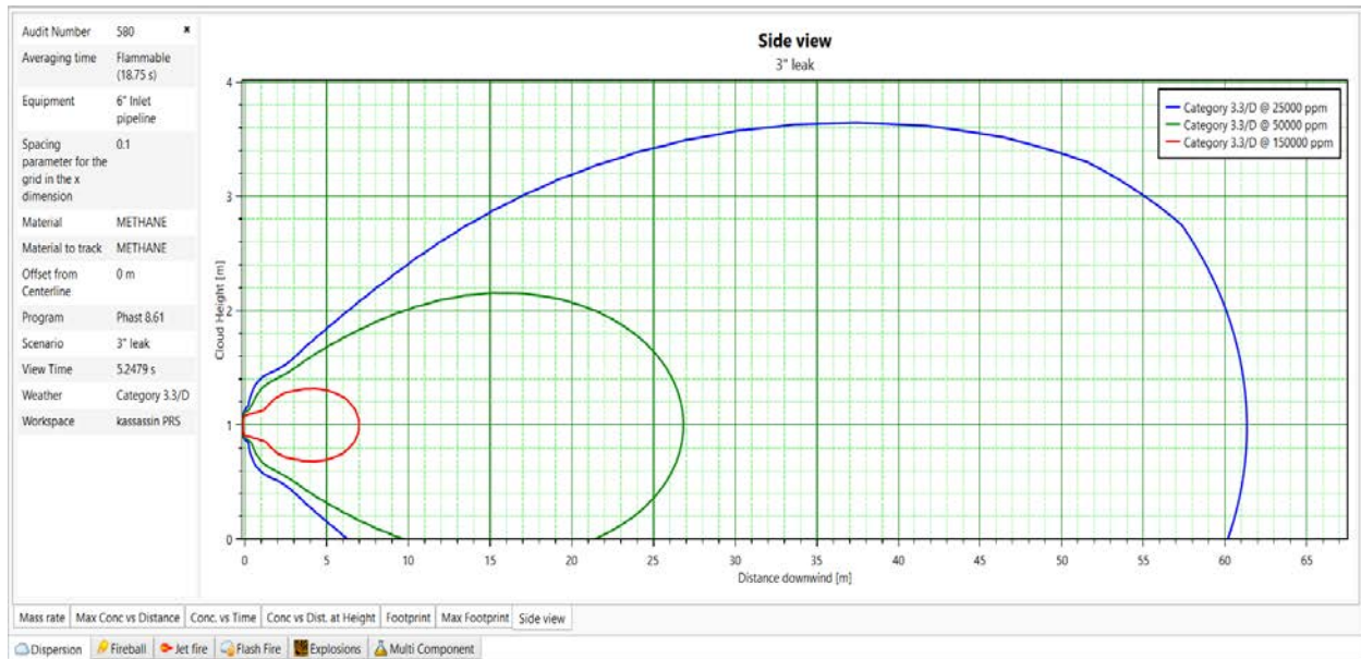
Figure 15. Gas Cloud Side View (UFL/LFL) (3" hole in 6" Inlet Pipeline)
