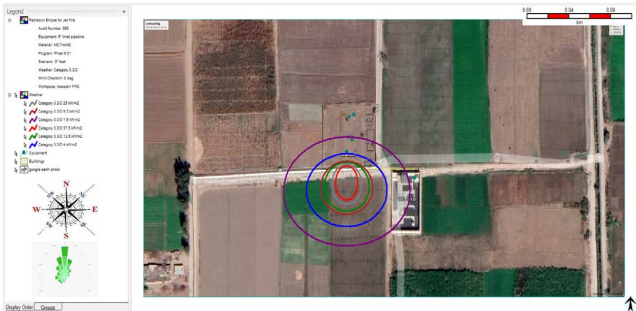
Figure 16. Heat Radiation Contours from Jet Fire (3" hole in 6" Inlet Pipeline)
