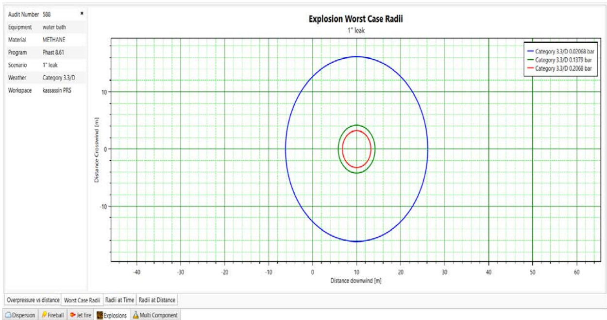
Figure 39. Explosion Overpressure Waves Graph (Gas Heater)
