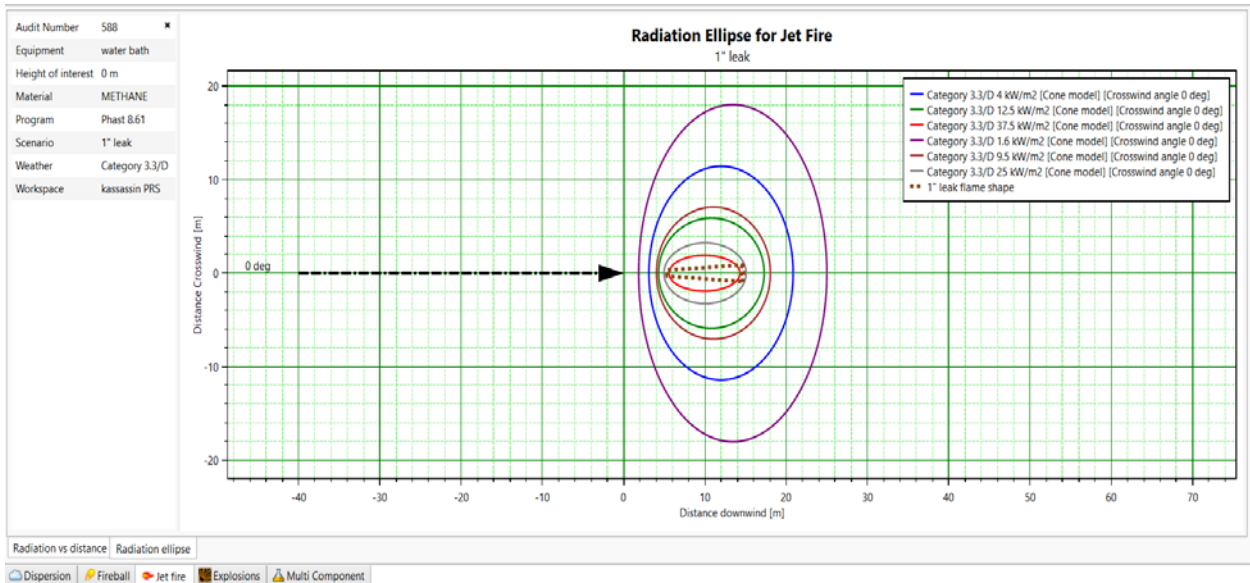
Figure 37. Heat Radiation Contours - Fire Graph (Gas Heater)
