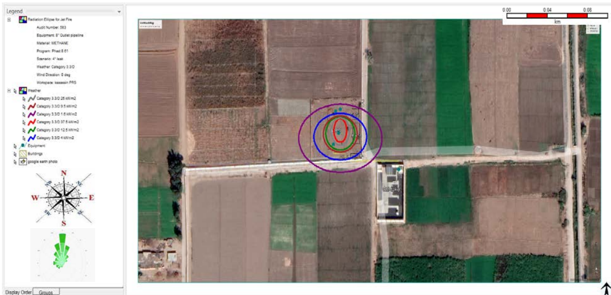
Figure 24. Heat Radiation Contours from Jet Fire (4'' hole in 8'' Outlet Pipeline)
