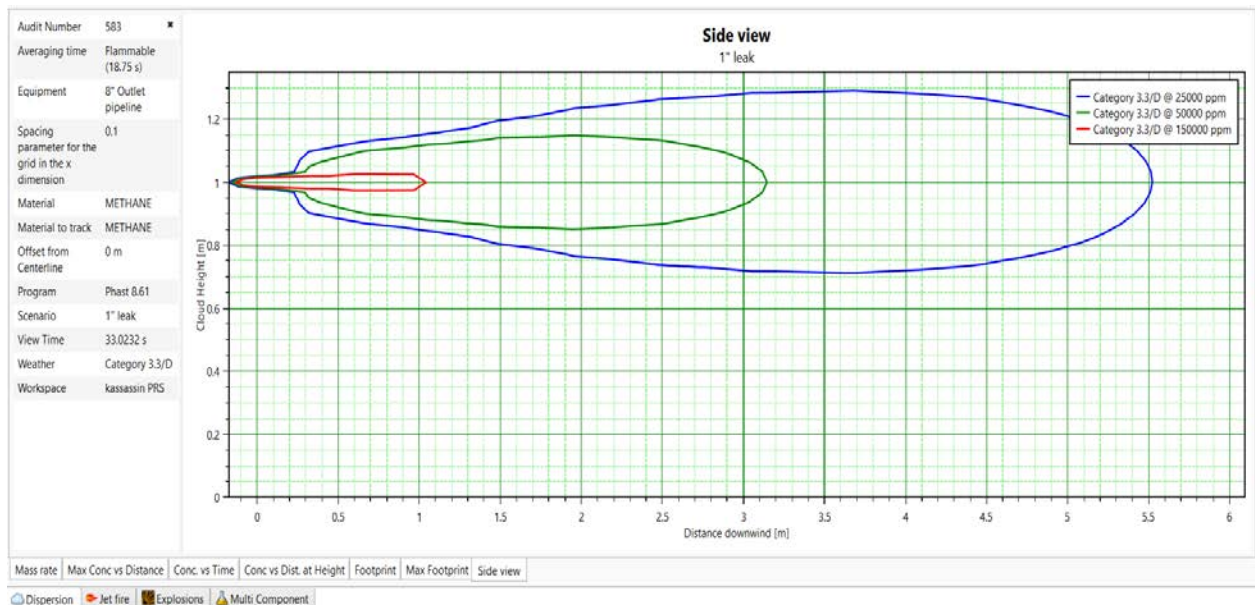
Figure 21. Gas Cloud Side View (UFL/LFL) (1" hole in 8" Outlet Pipeline)
