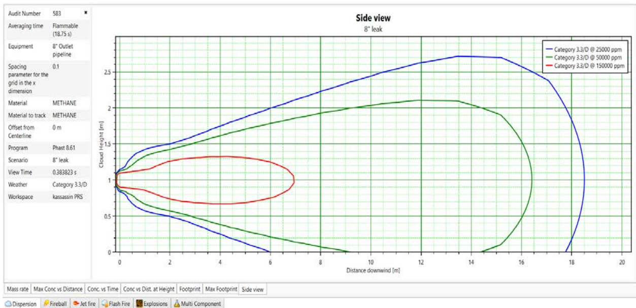
Figure 26. Gas Cloud Side View (UFL/LFL) (8'' Outlet Pipeline Full Rupture)
