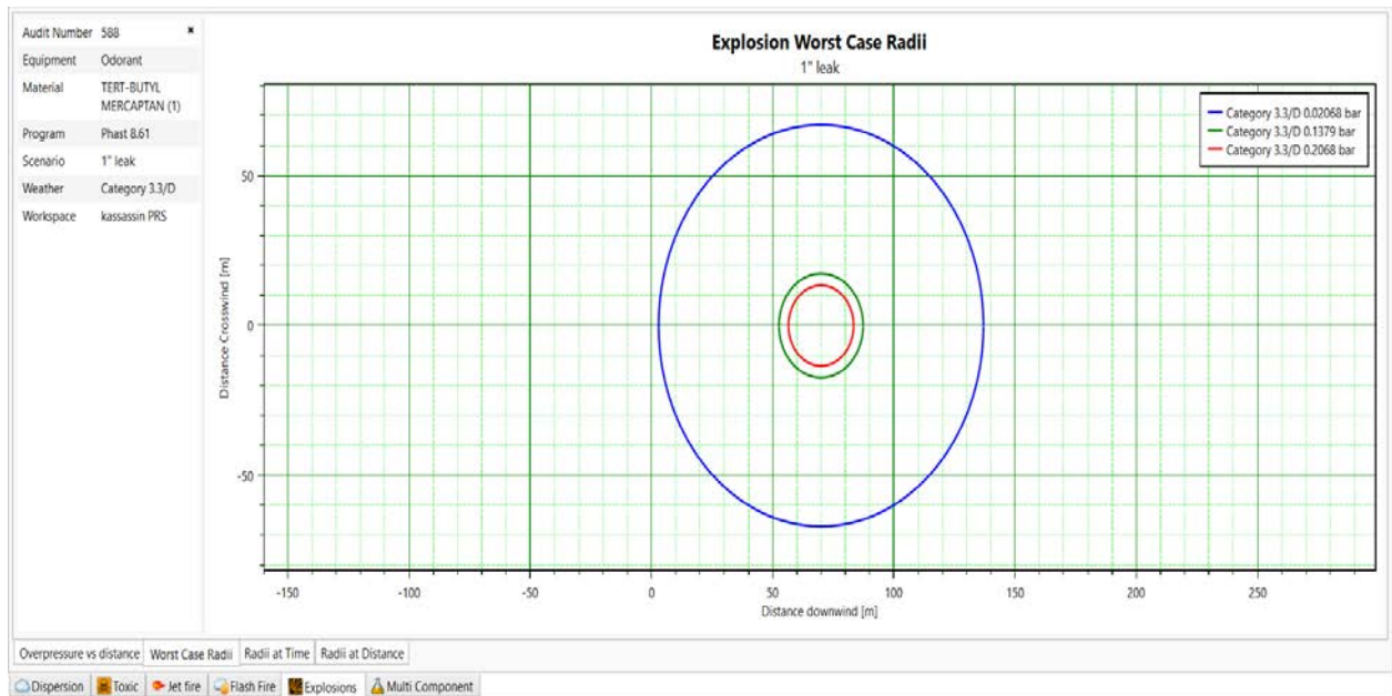
Figure 34. Worst-Case Explosion Overpressure Waves Graph (Odorant Leak)
