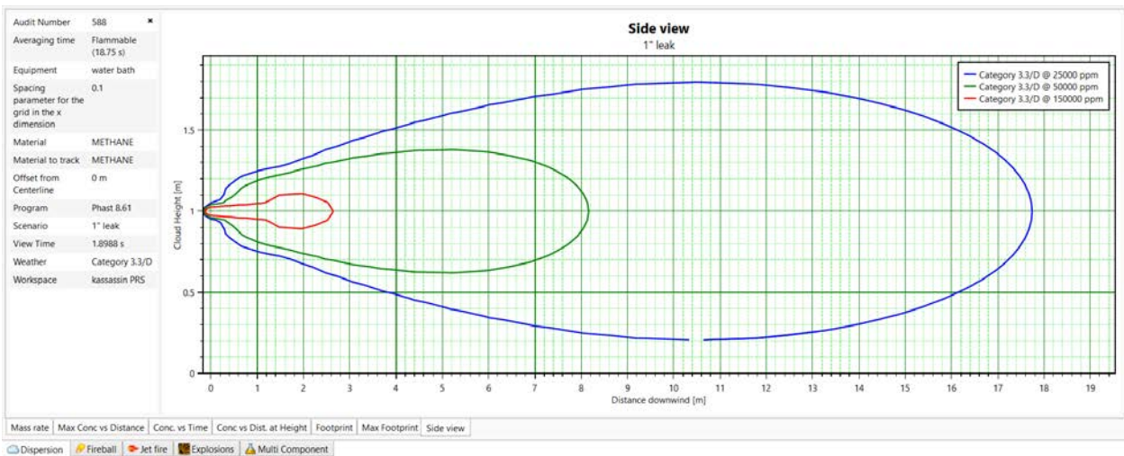
Figure 36. Vapor Cloud (UFL/LFL) Side View Graph (Gas Heater)
