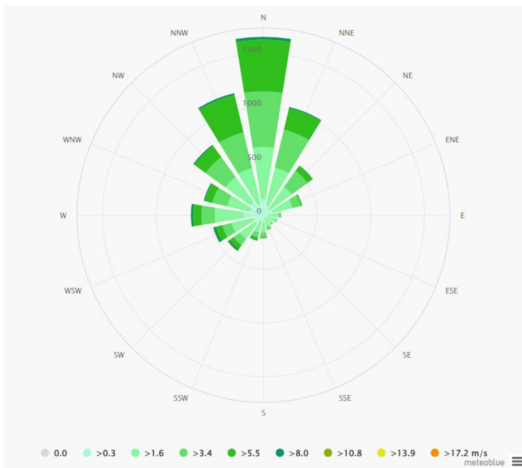
Figure 6. Wind Rose for El- Kasasin Area
