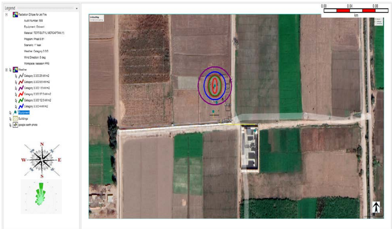
Figure 33. Heat Radiation Contours - Jet Fire on Site (Odorant Leak)
