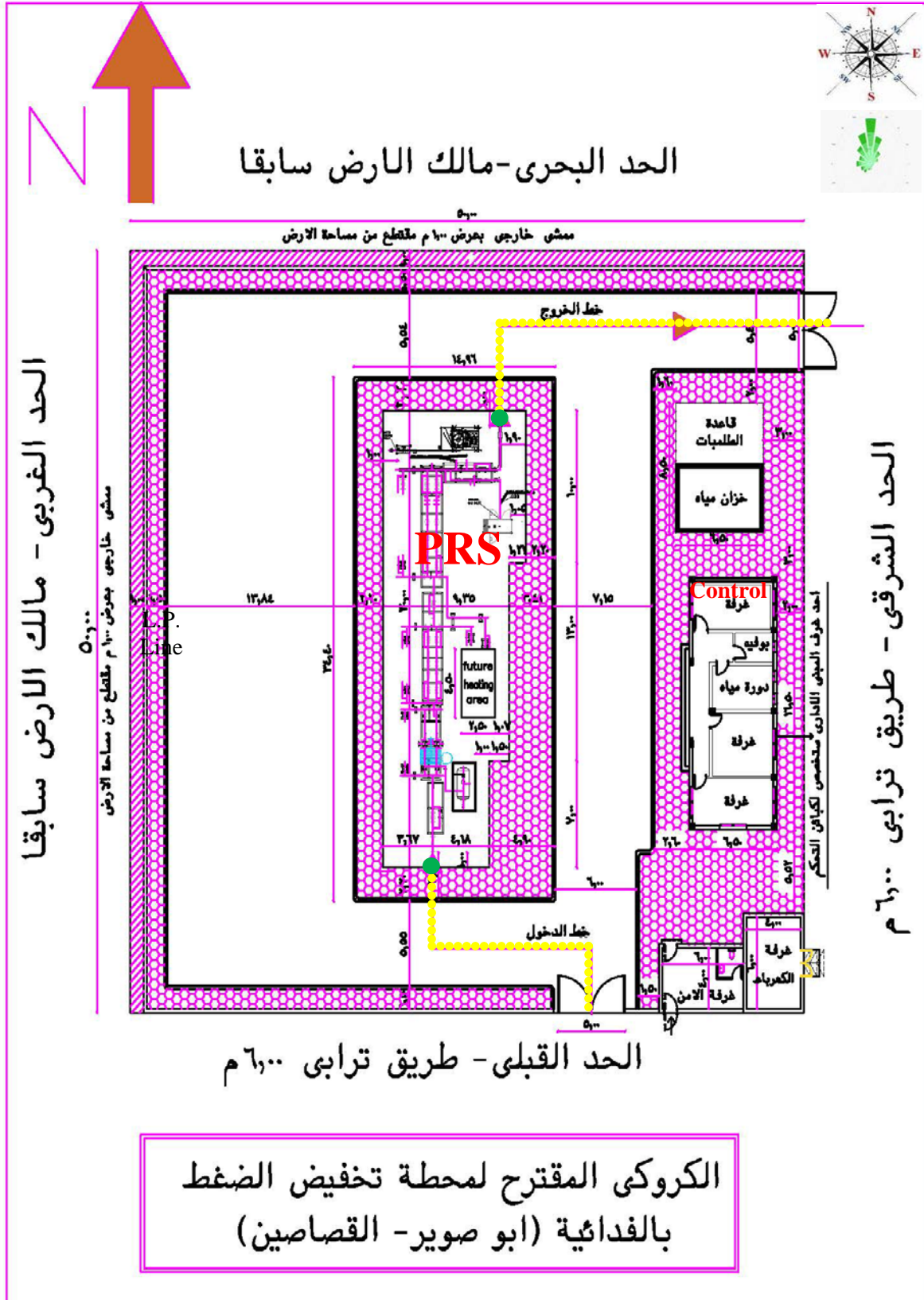
Figure 8. El- Kasasin PRMS Layout
