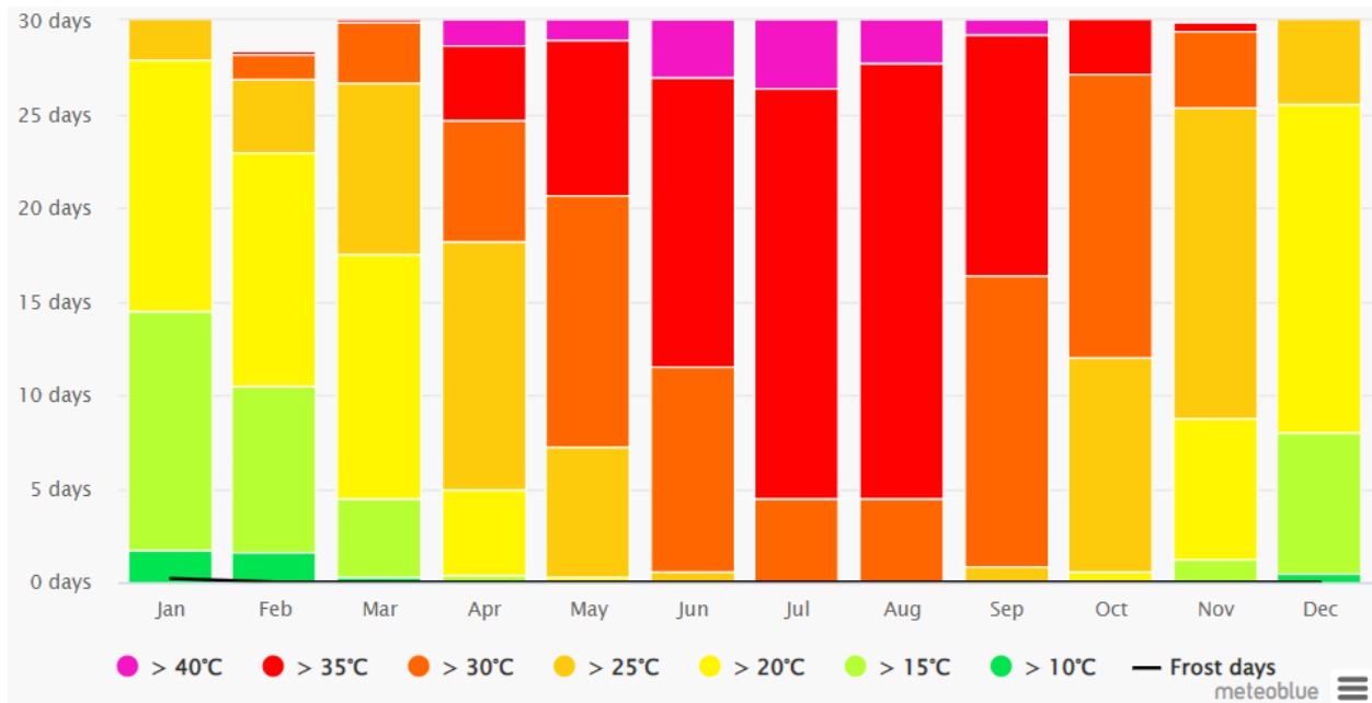
Figure 4. Monthly Variations of the Maximum Temperature for El- Kasasin Area
