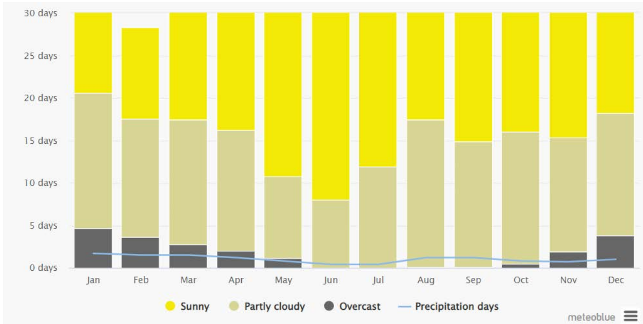
Figure 7. Monthly Variations of the Sunny, Cloudy and Precipitation days for El- Kasasin Area
